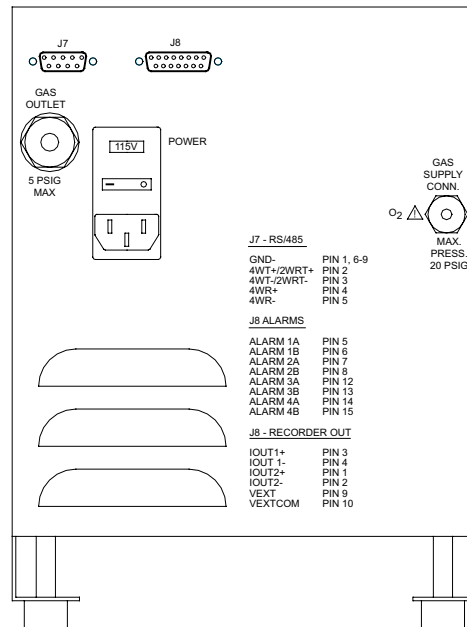
Rear Panel of CG1000 Analyzer
