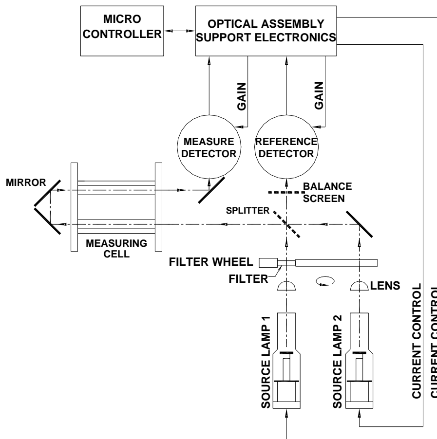
Figure 2 – Dual Beam Multi-Wavelength Spectrophotometer
