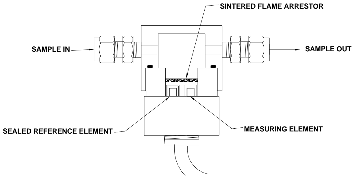
Figure 3 – Layout of Thermal Conductivity Sensor
