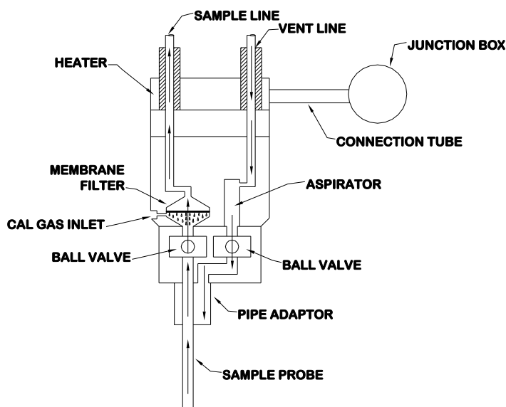
Figure 5 – Schematic of Heated Sample Probe
